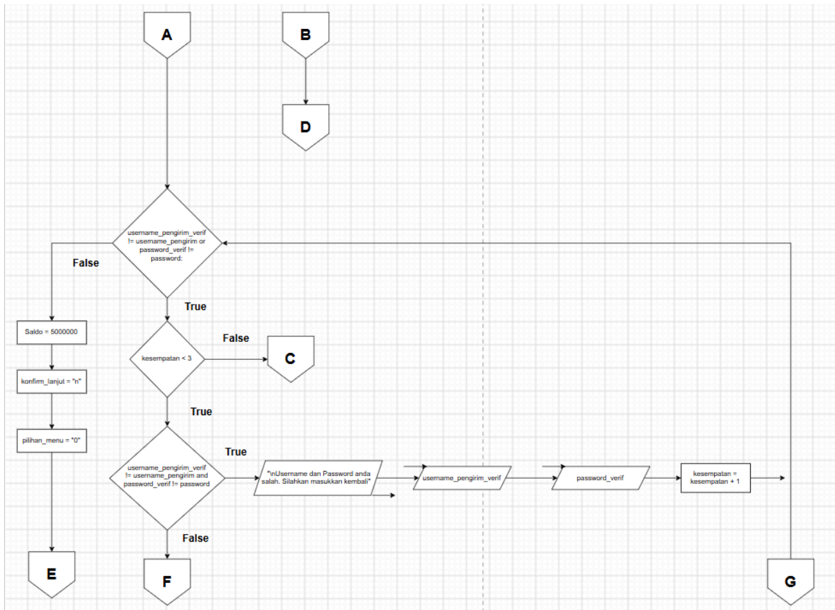
Gambar 1.2 Flowchart Halaman 2
