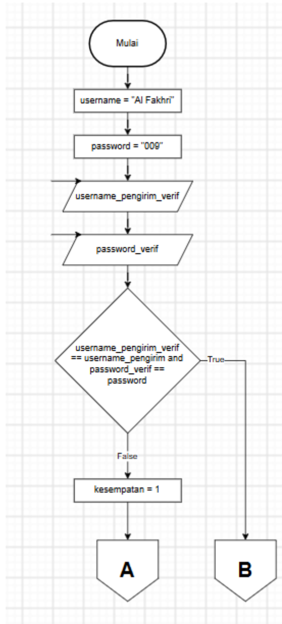
Gambar 1.1 Flowchart Halaman 1
