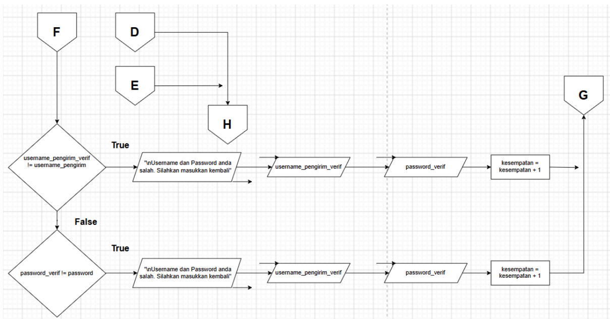
Gambar 1.3 Flowchart Halaman 3
